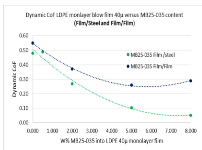
Figure 1: Dynamic CoF monolayer 40 \mu LDPE blown film versus Dow Corning MB25-035 Masterbatch content, %.
